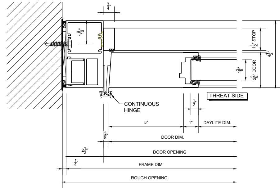
5 DOOR JAMB DETAIL (HINGE) SCALE: 3" = 1'-0"
