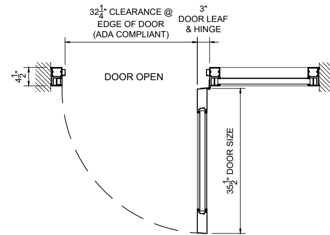
SINGLE DOOR FRAME PLAN
