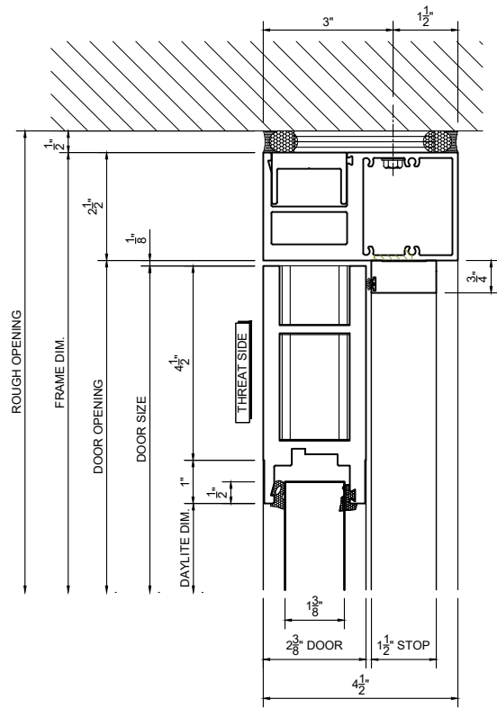
1 DOOR HEAD DETAIL SCALE: 3" = 1'-0"
