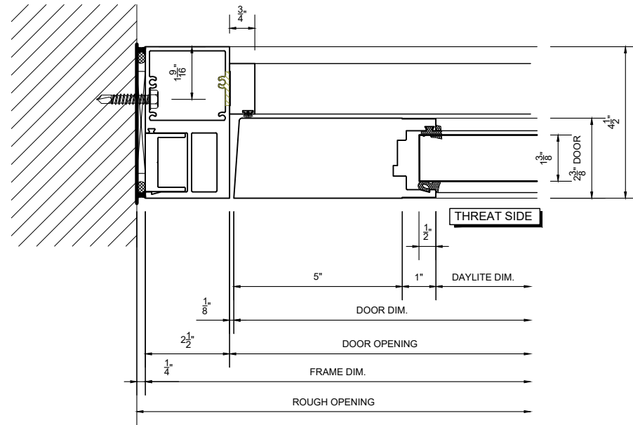
3 DOOR JAMB DETAIL (STRIKE) SCALE: 3" = 1'-0"
