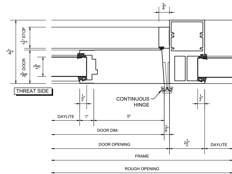
6 DOOR @ HINGE TO JAMB W/ SIDELITE SCALE: 3" = 1'-0"
