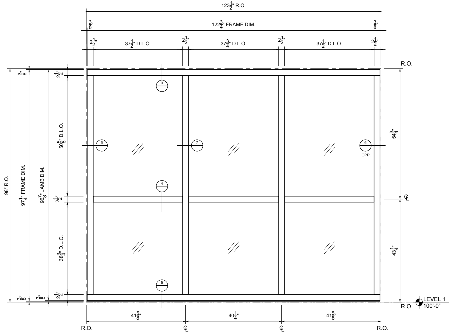
1 INTERIOR FRAME ELEVATION SCALE: 1/2" = 1'-0"
