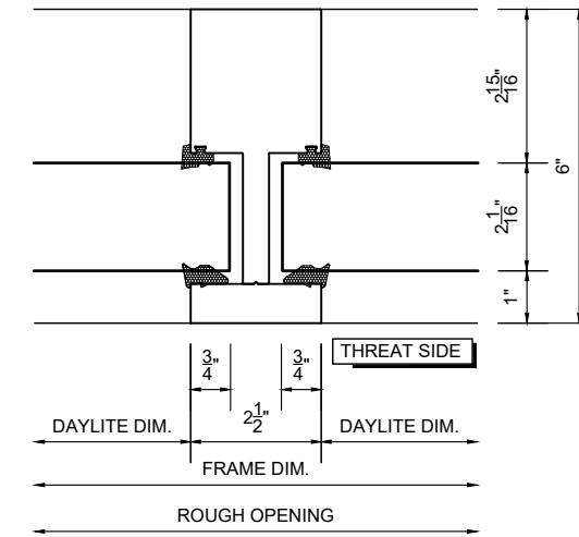
7 VERT. MULLION DETAIL SCALE: 3" = 1'-0"
