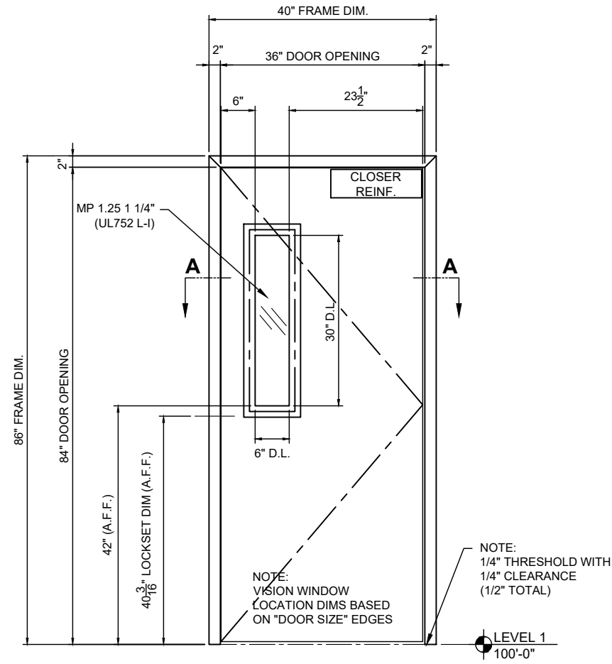
1 SINGLE DOOR ELEVATION SCALE: 1/2" = 1'-0"
